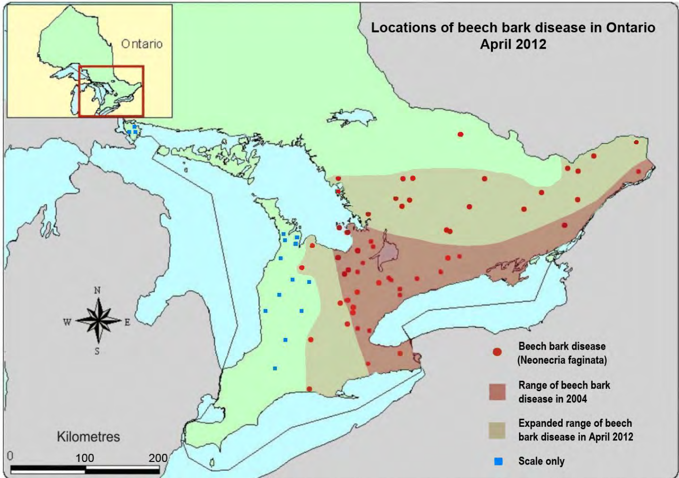
Figure 9. The range of beech bark disease in Ontario as of spring 2012, showing progression since 2004 and locations of scale-only infestations. The lone red dot in the upper right is considered a satellite disease centre – an area to which the disease was transported, possibly via movement of firewood.
